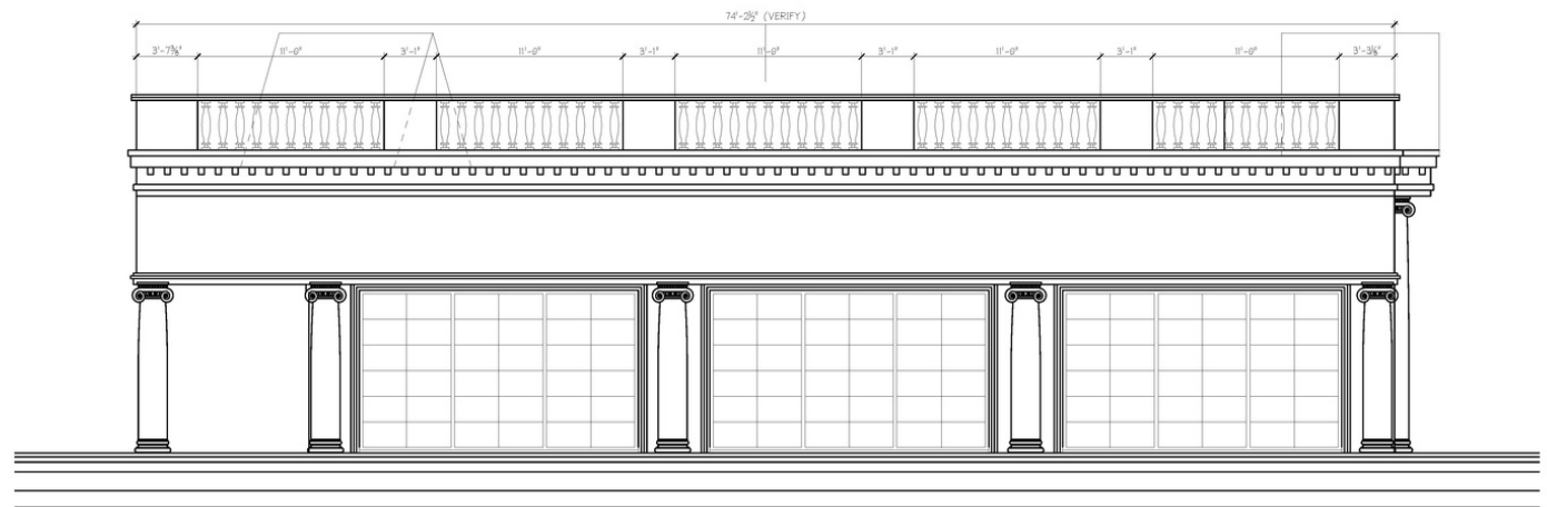
WEST ELEVATION
