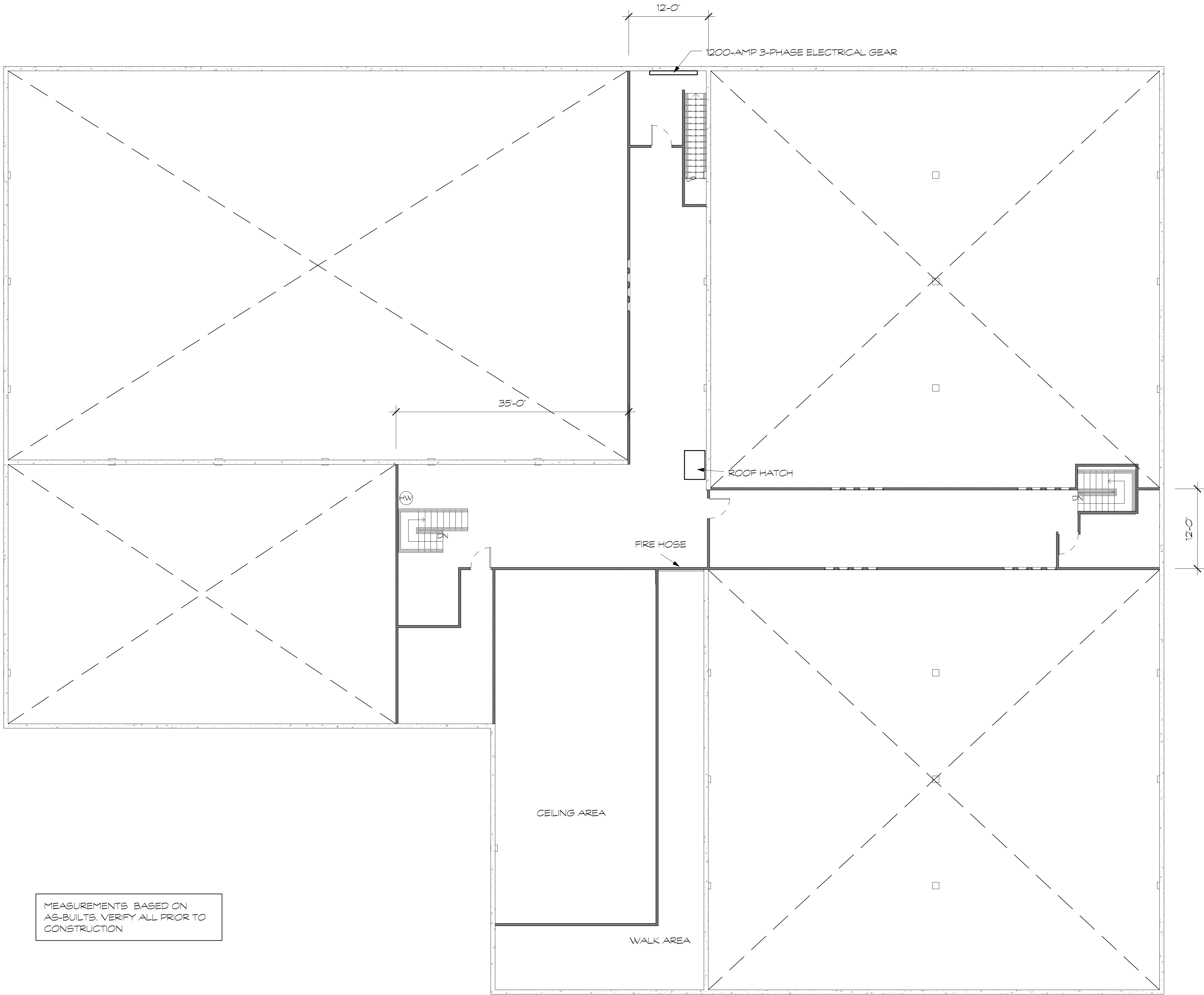
1 UPPER LEVEL FLOOR PLAN SCALE: 1/8" = 1'-0"
